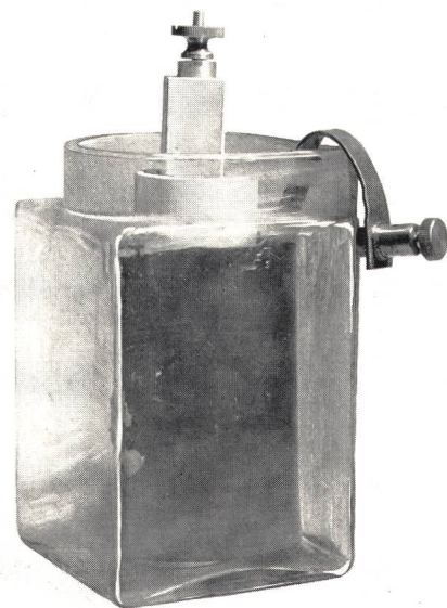
Fig. 2 Daniell-Element
