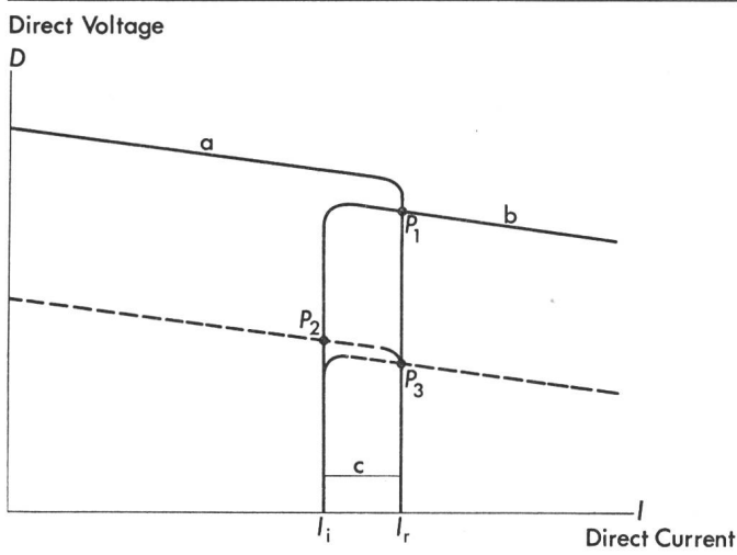
Fig. 3 Control Curve
