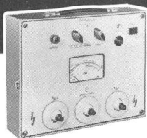
A-1807 HS-Isolationsmesser, Akku/Netz 1000 - 2500 - 5000 V DC, 40 kΩ ... 100 GΩ
