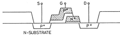
TETRODE WITH WRITING BY FOWLER-NORDHEIM EMISSION
