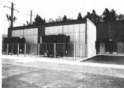
Fig. 3 BKW/IBB-Unterstation Heimiswil
