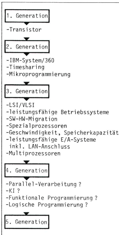
Figur 7 Computergenerationen
