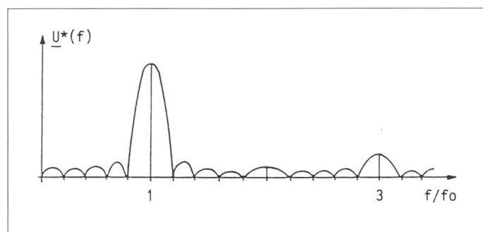
Figure 8 Spectre de la tension
