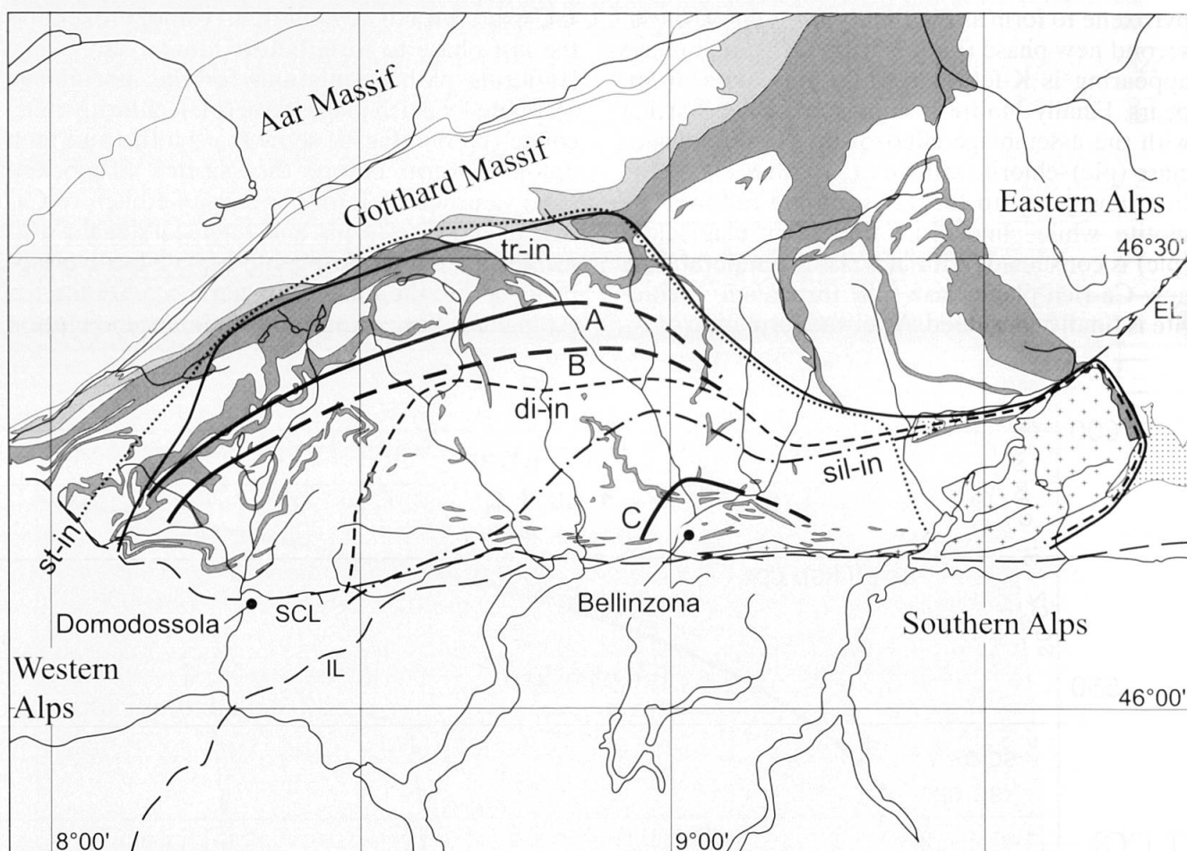
Fig. 10 Schematic map of the Central Alps from Fig. 1 showing the approximate geographic location of the transition clinozoisite + plagioclase to scapolite-bearing assemblages (A), the appearance of K-feldspar (B) and the appearance of clinopyroxene (C) in calc-schists, superimposed on the Geological map of Switzerland (1980).
