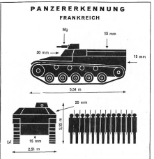
SCHEMATA PANZERKENNUNG ARKA V.T.P. (Schemata of tank identification device ARKA V.T.P.)
