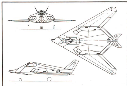
Three View Aktuell US Air Force/Tactical Air Command/Lockheed Stealth-Luftangriffsflugzeug F-117A (Codennamen: Have
