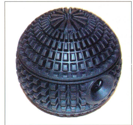
Short Range Throwing Camera von Defence Optical Systems
