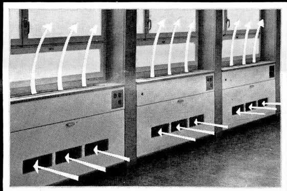
Air Conditioning Convector, built in type as installed on the Continent and similar to the ones installed in the B. A. S. F. building in Ludwigshafen as illustrated.
