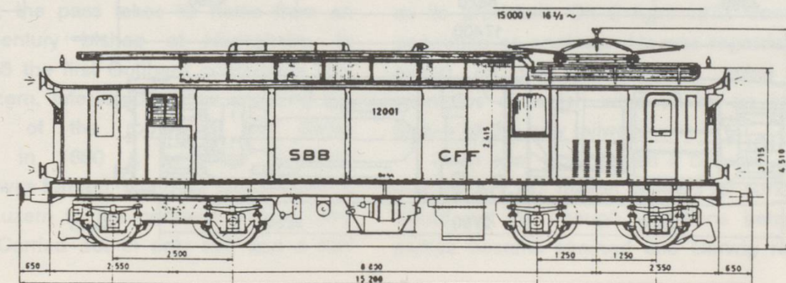
Figure 2 Be4/4 No.12001
