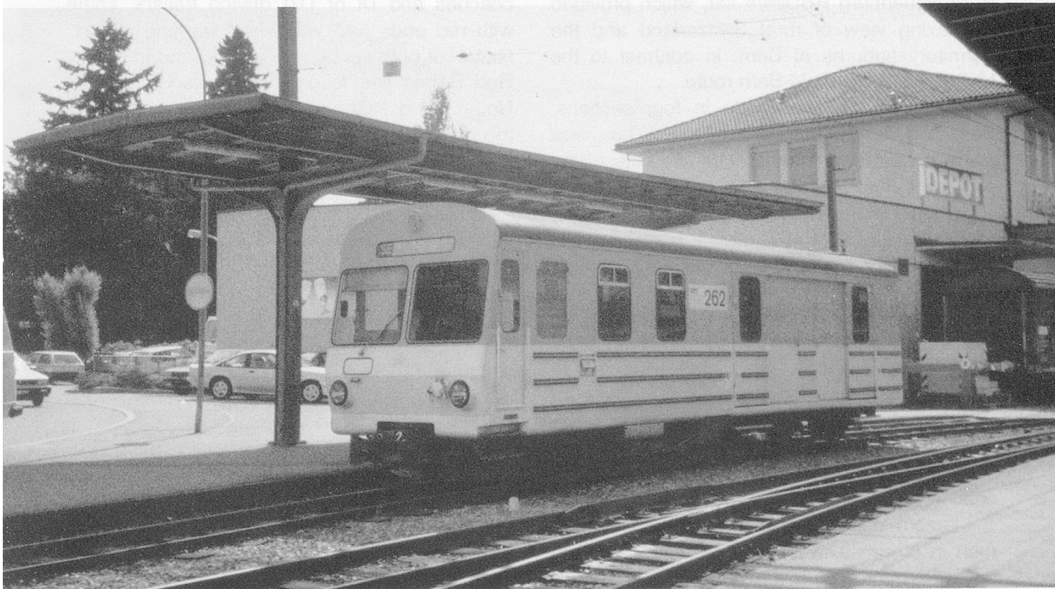
Below: RBS PTT Zt driving trailer No.262 at Solothurn, 4 July 1989. To the right is the Feldschlössen Bier depot with Hbis 21 85 225 0 420-6.
