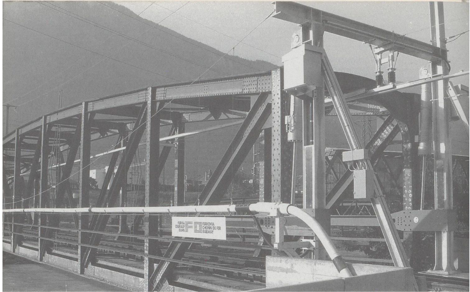
Furka-Oberalp Above & Below: Views of the bridge between Brig and Naters which now lifts so that if the river floods no damage will be sustained and rail connections can be maintained.
