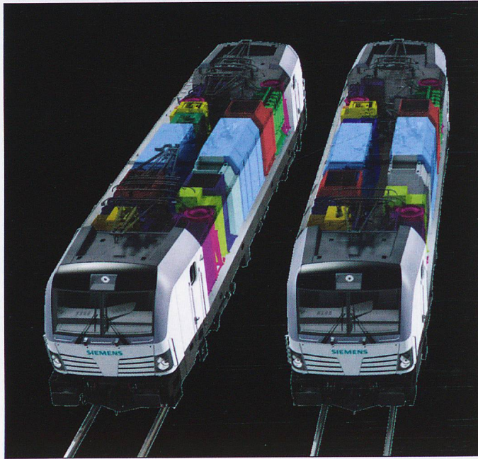
TOP: A drawing showing the Vectron Diesel Version - Siemens image. ABOVE: A drawing showing the Vectron MS and AC Versions - Siemens image. BELOW: railCare Vectron 476 452 passes Ausserberg - June 2018. BOTTOM: A Trix Model of PR 22095 BLS Cargo Vectron.
