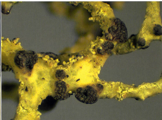
PHACOPSIS VULPINA
