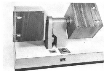
Pilling Tester
