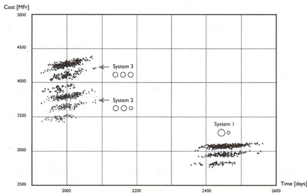
Fig. 12: GBT Systems Study – Resulting Cost-Time Scattergrams.
