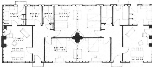
PLAN TYPE A BUNGALOW
