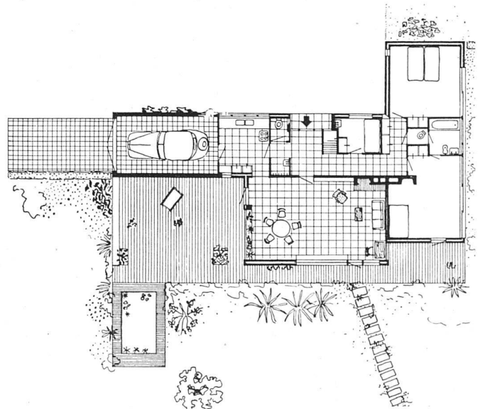
Grundriß 1:300 / Rez-de-chaussée / Ground floor plan
