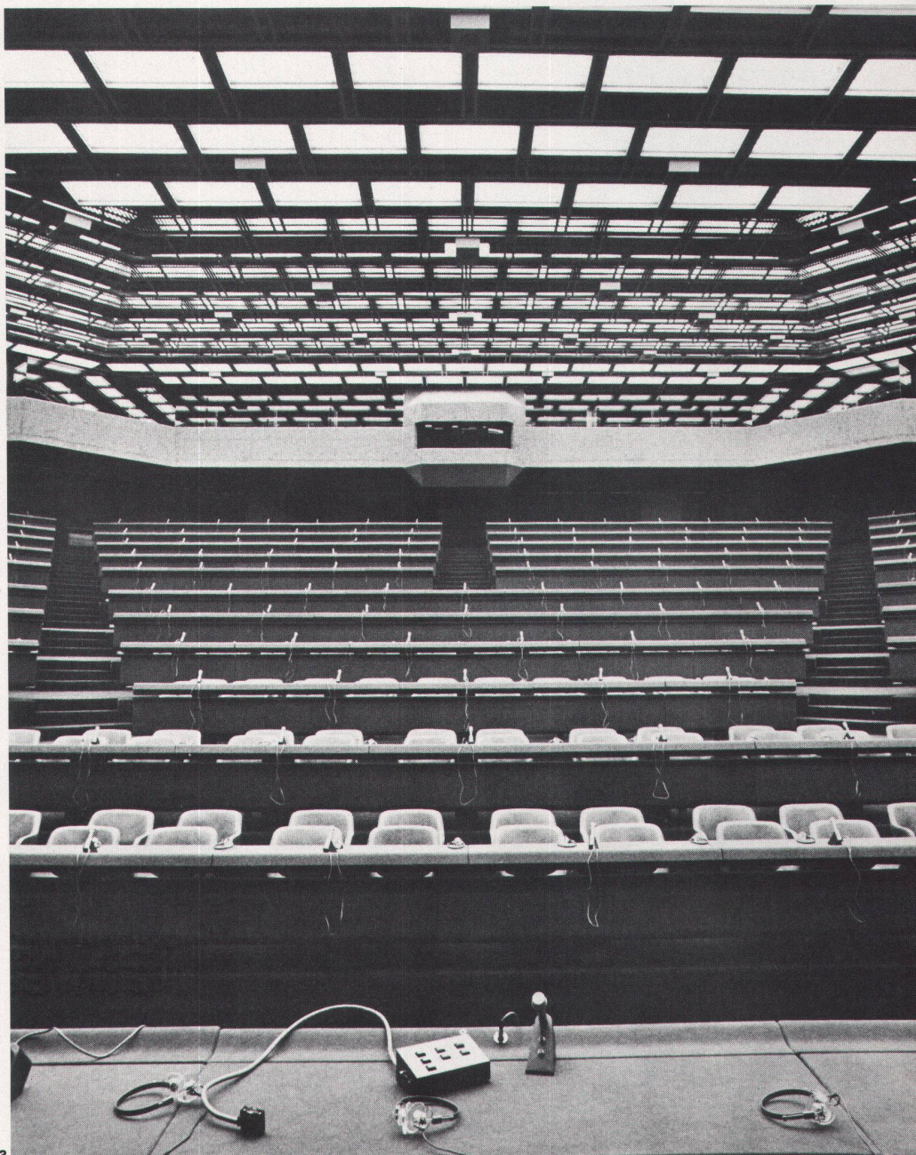
12 The large auditorium with inclined seating, capacity 800. The screen-wall and the podium can be retracted into the floor, making possible combination with the intermediate hall.
