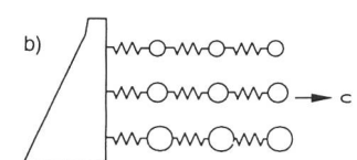
Halbunendliches Feder-Masse-System
